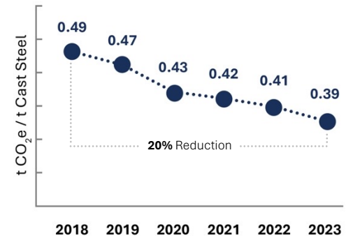
SDI Steel Mills' Scope 1 & 2 GHG Emissions Intensity 2
